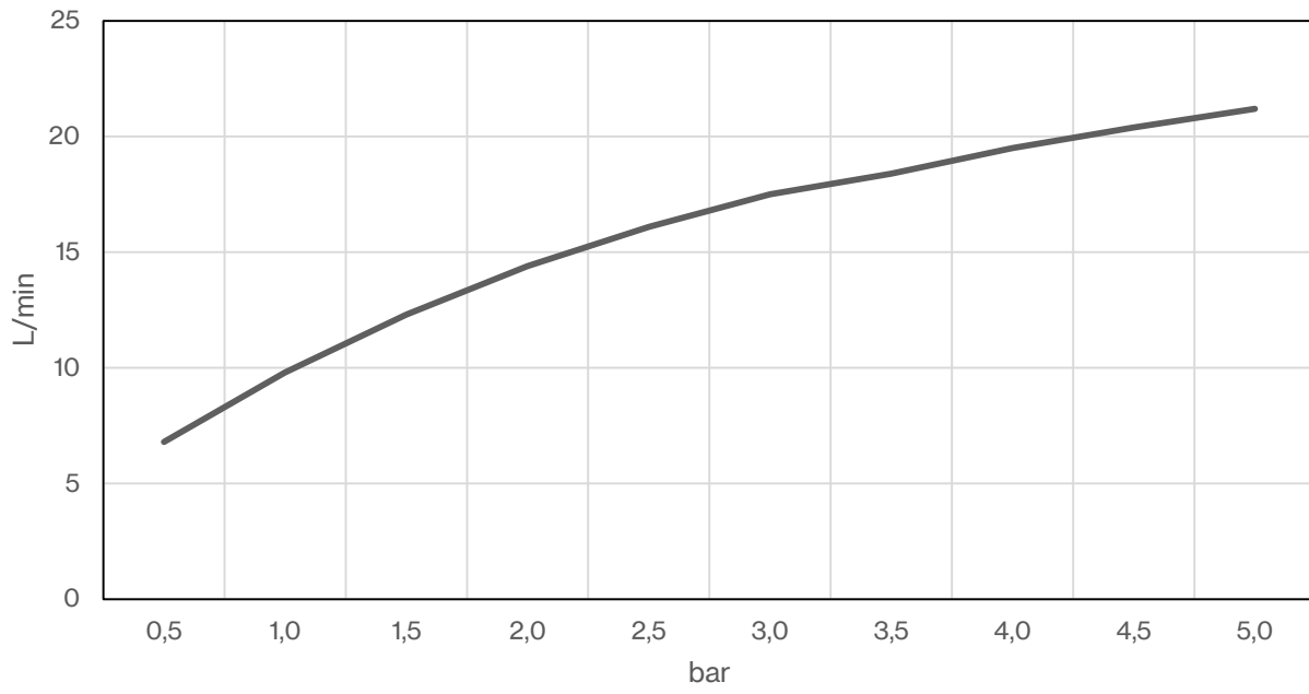
QA3190 flow rate (without aerator)
