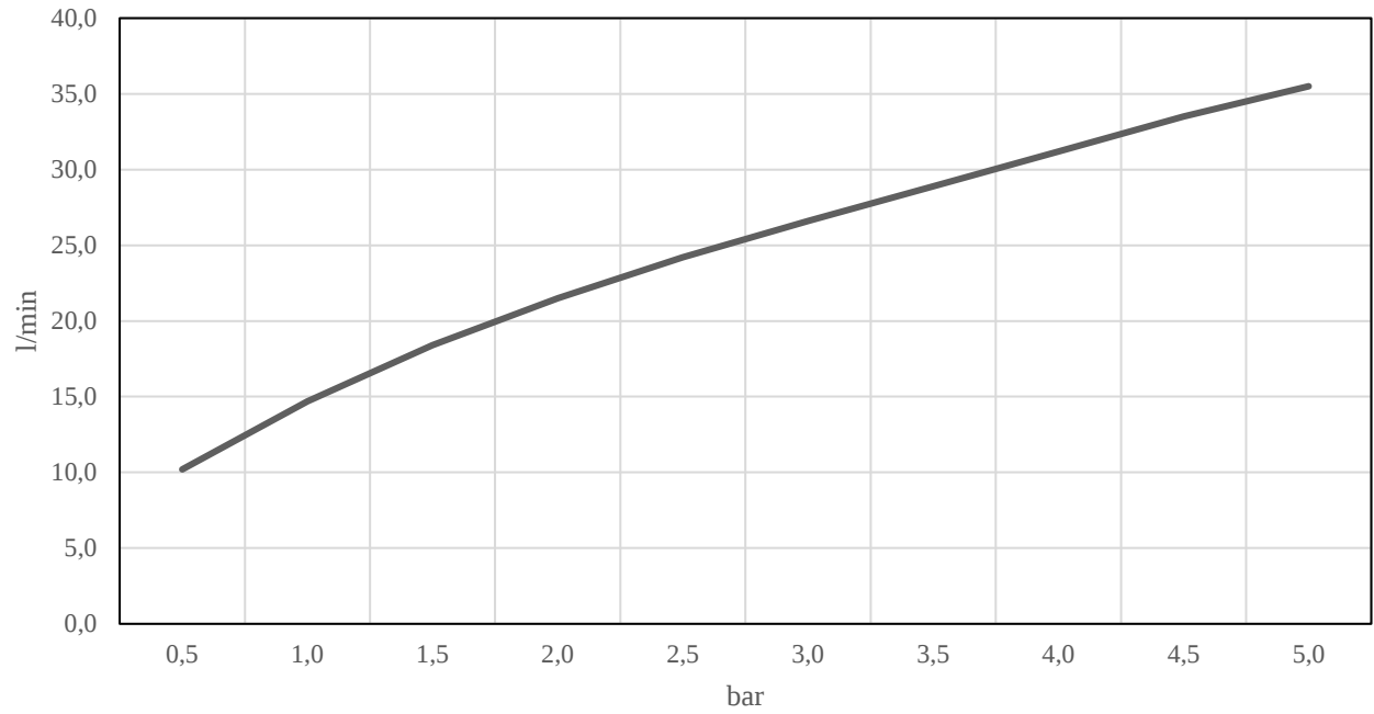
QS5110 flow rate (without aerator)
