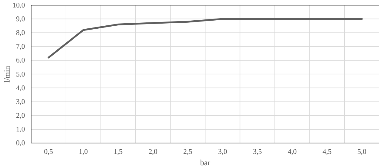
QS5110 flow rate (with aerator)
