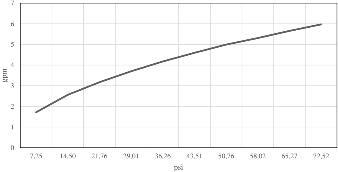
QS3300 flow rate(gpm)
